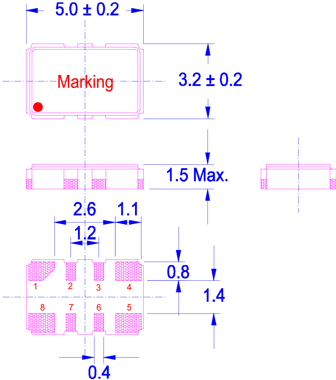
Package Drawing
