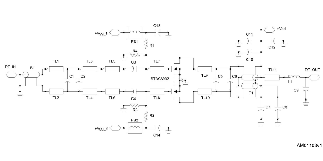
Figure 3. Electrical schematic
