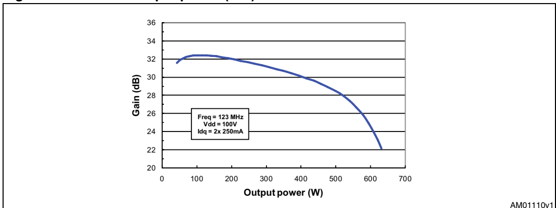
Figure 10. Gain vs output power (CW)
