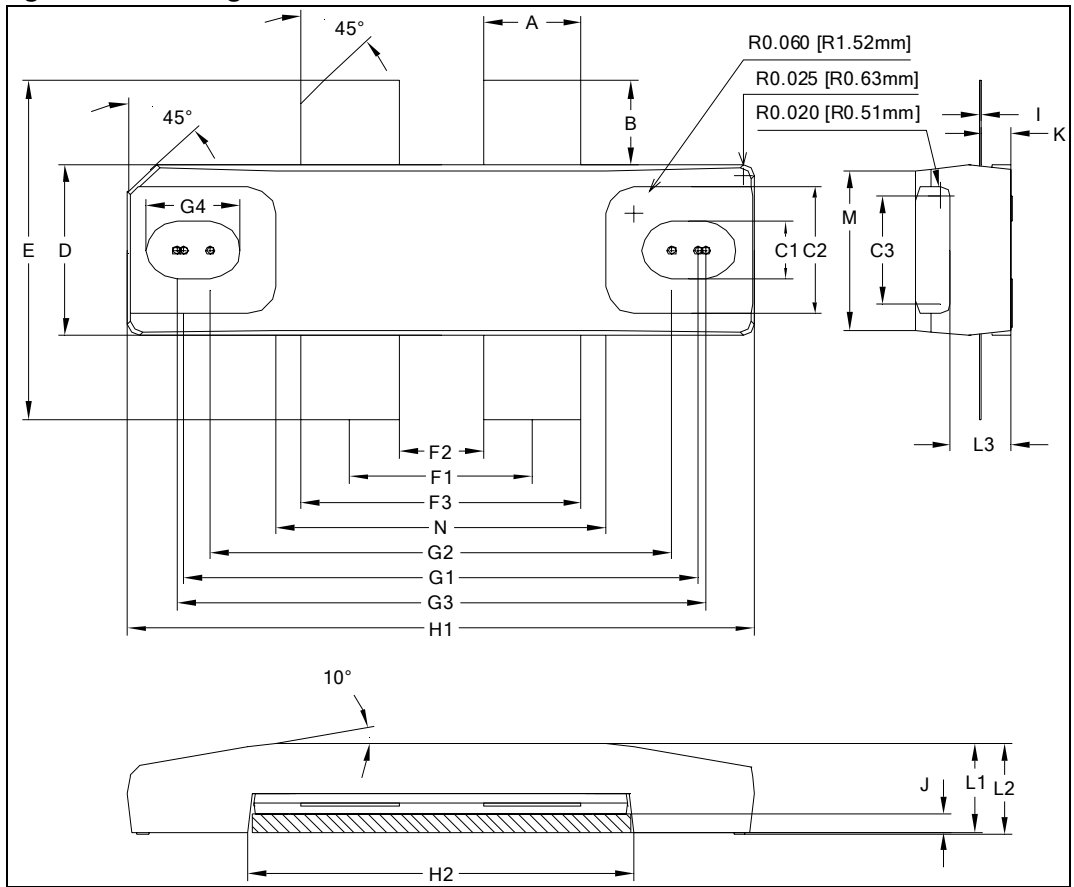
Figure 12. Package dimensions
