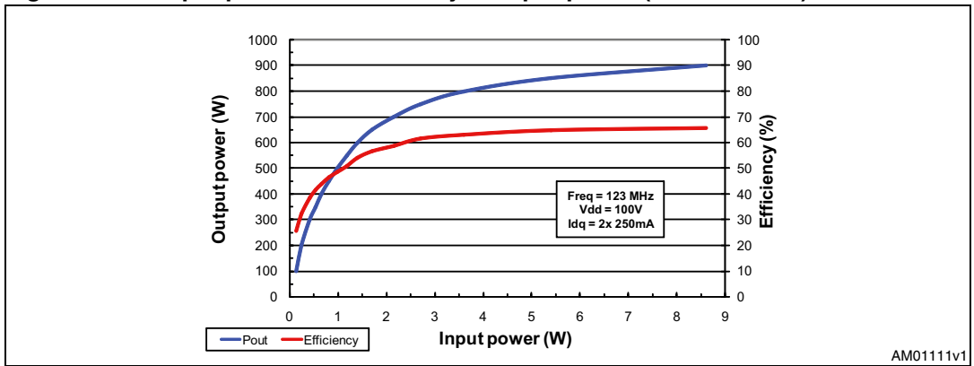
Figure 11. Output power and efficiency vs input power (1 msec - 10%)
